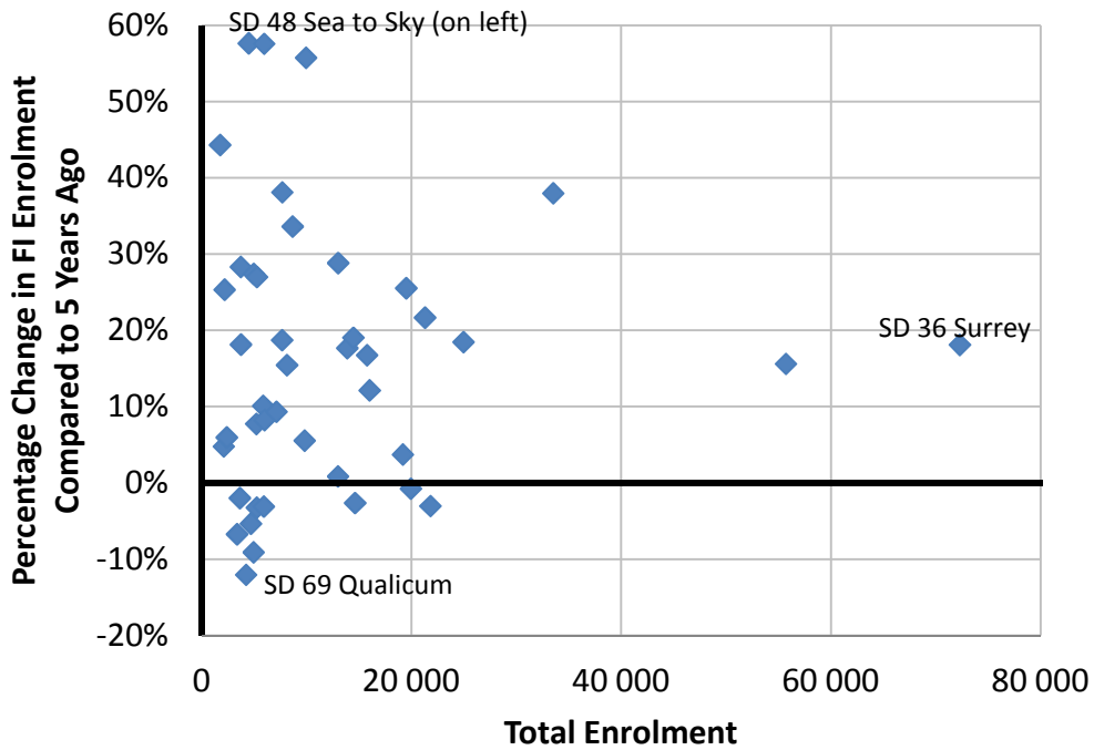
Figure 2. Percentage Change in FI Enrolment (2008/09–2013/14, 6 years) vs. Total Enrolment (2013/14). Outliers removed
