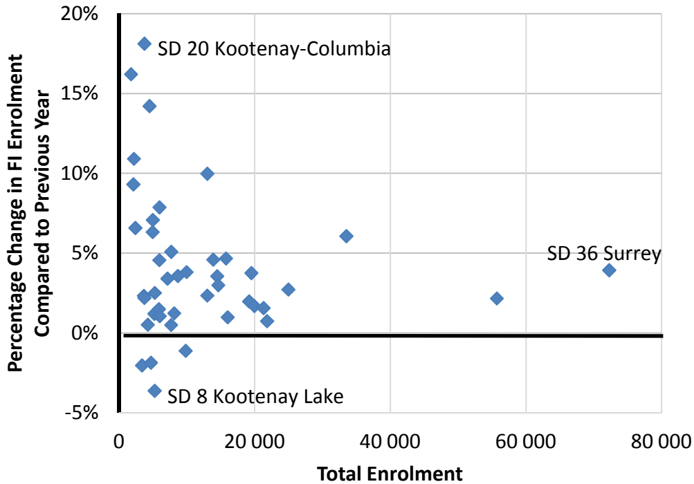
Figure 1. Percentage Change in FI Enrolment (2012/13–2013/14, 2 years) vs. Total Enrolment (2013/14). Outliers removed
