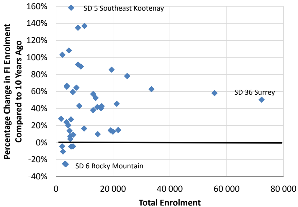
Figure 3. Percentage Change in FI Enrolment (2003/04-2013/14, 11 years) vs. Total Enrolment (2013/14). Outliers removed
